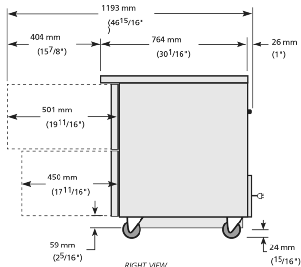
RIGHT VIEW
